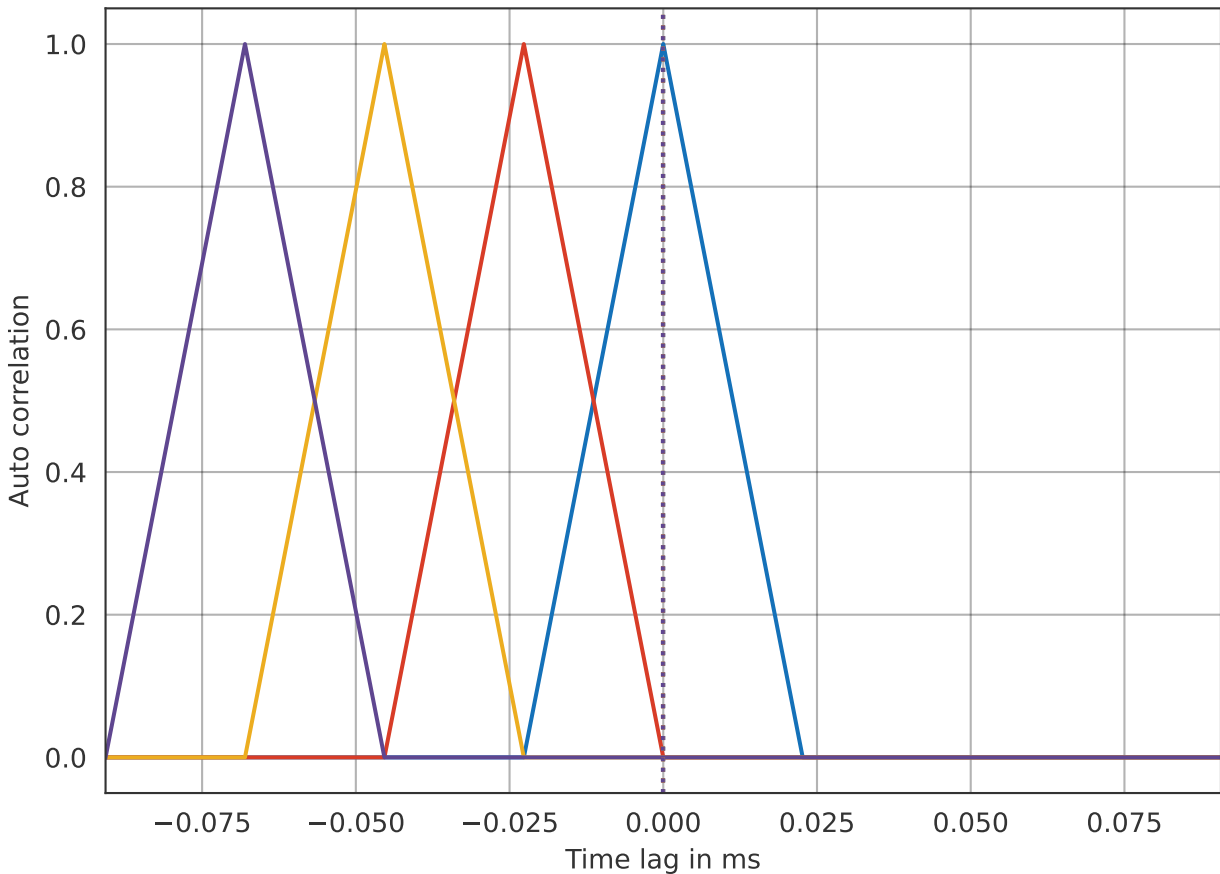
Correlation and position of maxima (dots)
