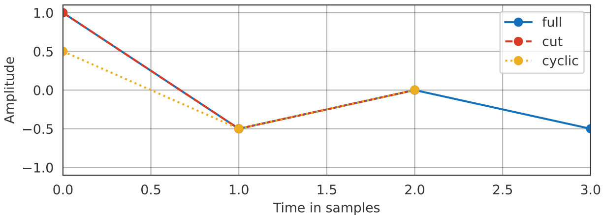
Convolution Result
